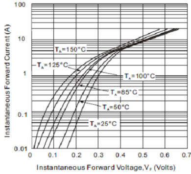
Fig. 1 - Instantaneous Forward Characteristics (per diode)
