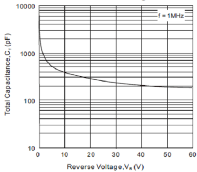
Fig. 5 - Total Capacitance VS. Reverse Voltage
