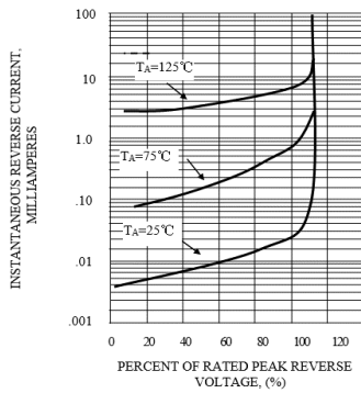
FIG. 3 - TYPICAL REVERSE CHARACTERISTICS
