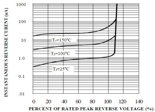
FIG. 3-TYPICAL REVERSE CHARACTERISTICS
