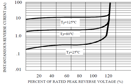
FIG. 3-TYPICAL REVERSE CHARACTERISTICS
