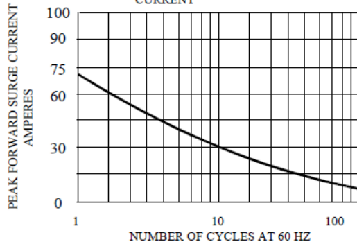
Fig. 4-MAXIMUM FORWARD SURGE CURRENT
