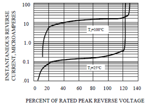
FIG. 3-TYPICAL REVERSE CHARACTERISTICS
