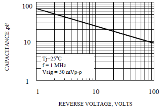
FIG. 5-TYPICAL JUNCTION CAPACITANCE
