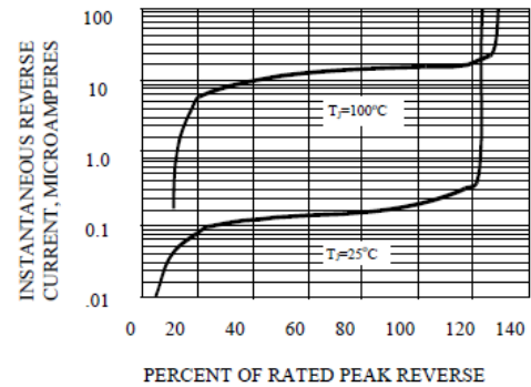
FIG. 3-TYPICAL REVERSE CHARACTERISTICS
