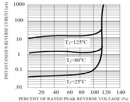
FIG. 3-TYPICAL REVERSE CHARACTERISTICS
