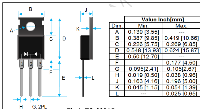
Fig 1. TO-220AB FOR MBR40U100CT
