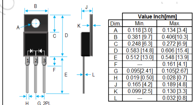
Fig 2. ITO-220AB FOR MBR40U100FCT
