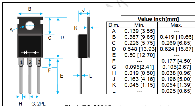
Fig 1. TO-220AB FOR MBR30U100CT
