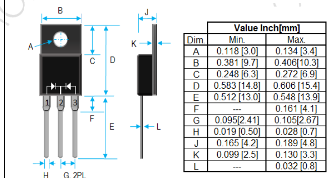
Fig 2. ITO-220AB FOR MBR30U100FCT
