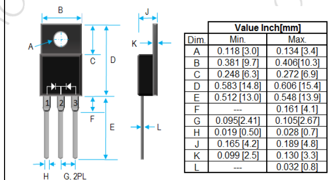
Fig 2. ITO-220AB FOR MBR30L120FCT
