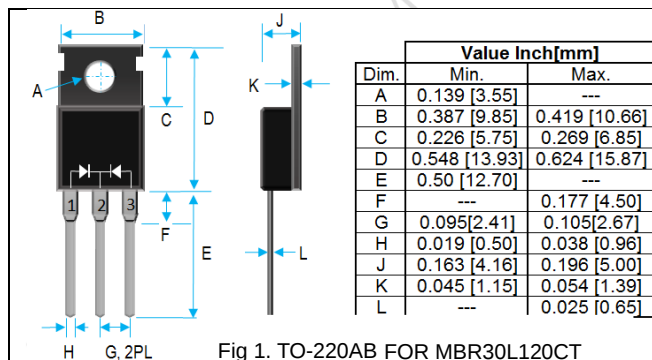
Fig 1. TO-220AB FOR MBR30L120CT
