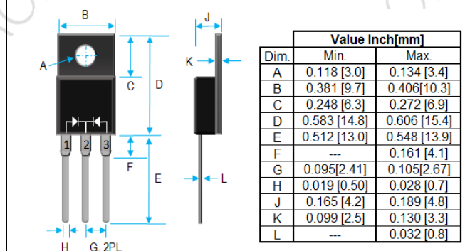
Fig 2. ITO-220AB FOR MBR30L100FCT
