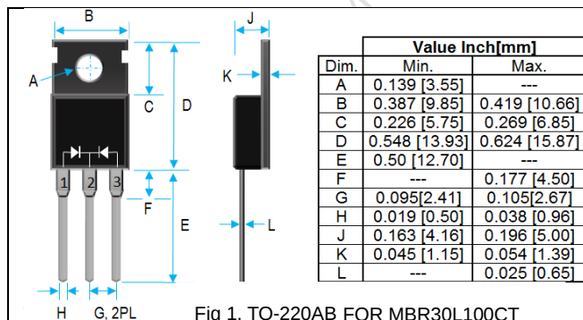
Fig 1. TO-220AB FOR MBR30L100CT
