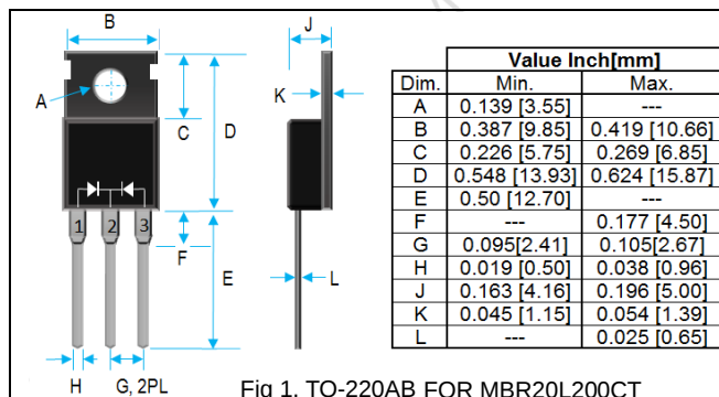
Fig 1. TO-220AB FOR MBR20L200CT
