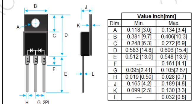
Fig 2. ITO-220AB FOR MBR20L200FCT
