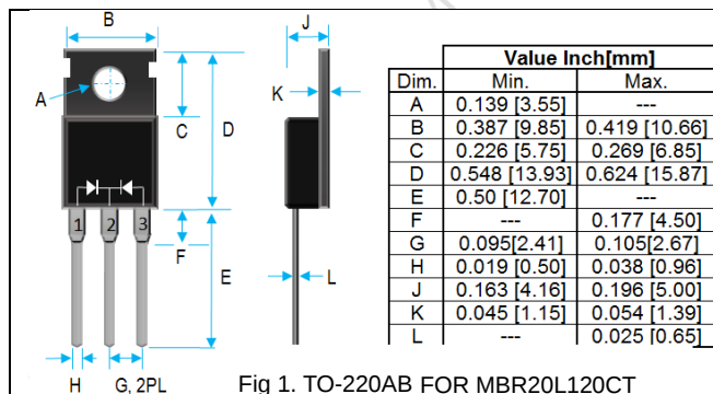
Fig 1. TO-220AB FOR MBR20L120CT
