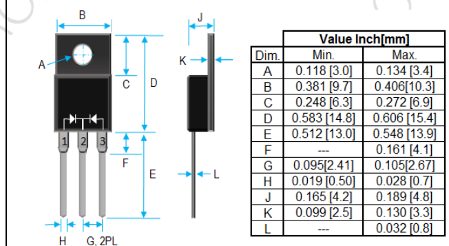
Fig 2. ITO-220AB FOR MBR20L120FCT
