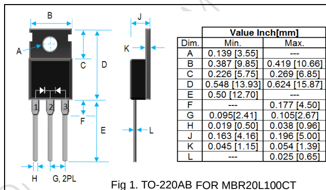
Fig 1. TO-220AB FOR MBR20L100CT
