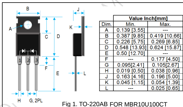
Fig 1. TO-220AB FOR MBR10U100CT
