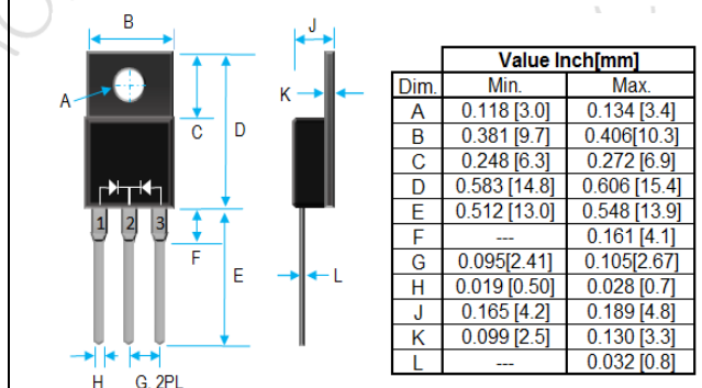
Fig 2. ITO-220AB FOR MBR10U100FCT
