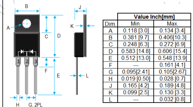
Fig 2. ITO-220AB FOR MBR10L45FCT
