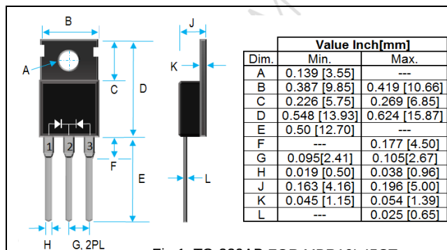
Fig 1. TO-220AB FOR MBR10L45CT
