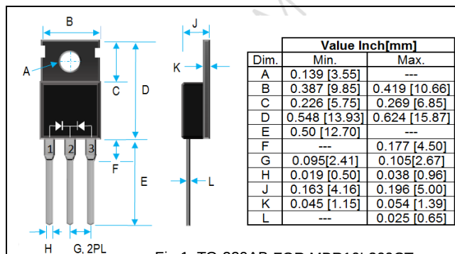
Fig 1. TO-220AB FOR MBR10L200CT
