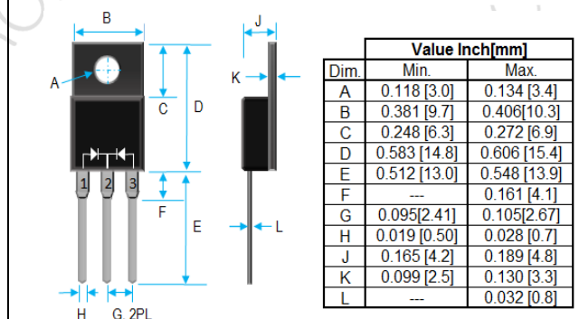
Fig 2. ITO-220AB FOR MBR10L100FCT
