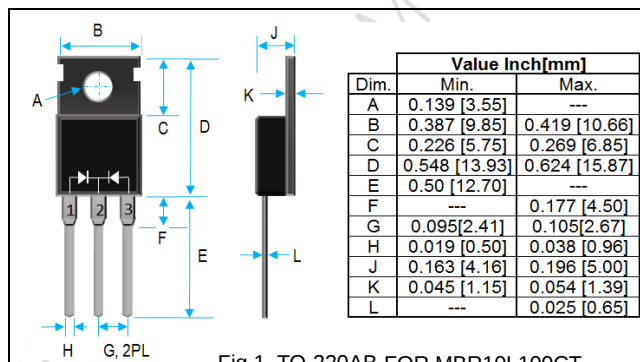
Fig 1. TO-220AB FOR MBR10L100CT
