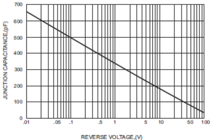
FIG.4-TYPICAL JUNCTION CAPACITANCE
