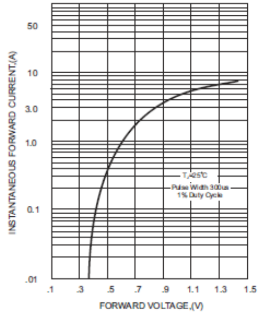
FIG.2-TYPICAL FORWARD CHARACTERISTICS
