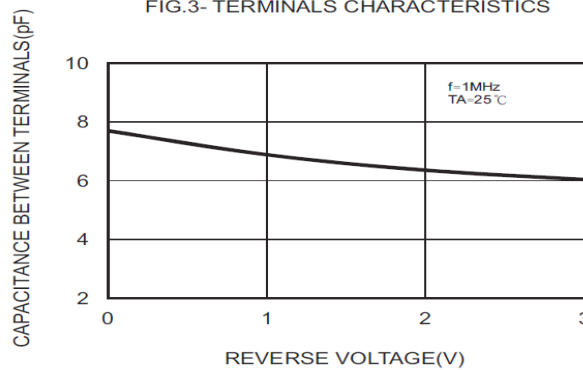
FIG.3- TERMINALS CHARACTERISTICS
