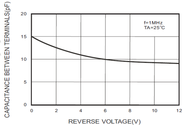
FIG.3- TERMINALS CHARACTERISTICS
