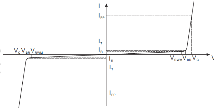
Bi-Directional TVS
