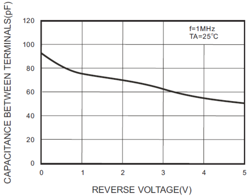
FIG.3- TERMINALS CHARACTERISTICS
