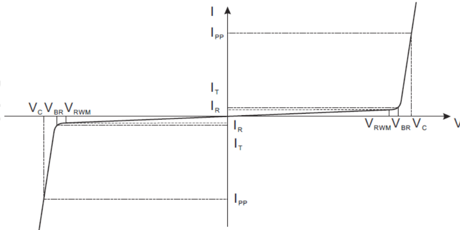
Bi-Directional TVS
