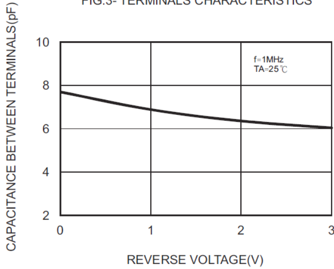
FIG.3- TERMINALS CHARACTERISTICS
