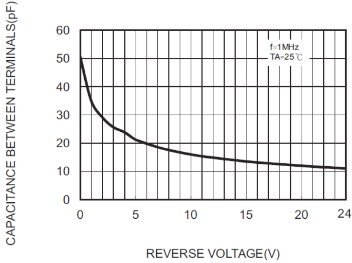
FIG.3- TERMINALS CHARACTERISTICS
