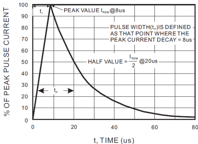
FIG.1- 8 X 20us PULSE WAVEFORM
