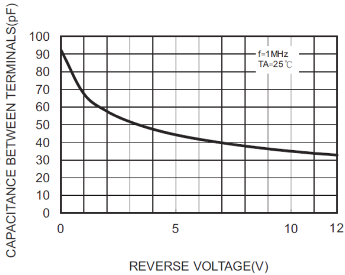
FIG.3- TERMINALS CHARACTERISTICS
