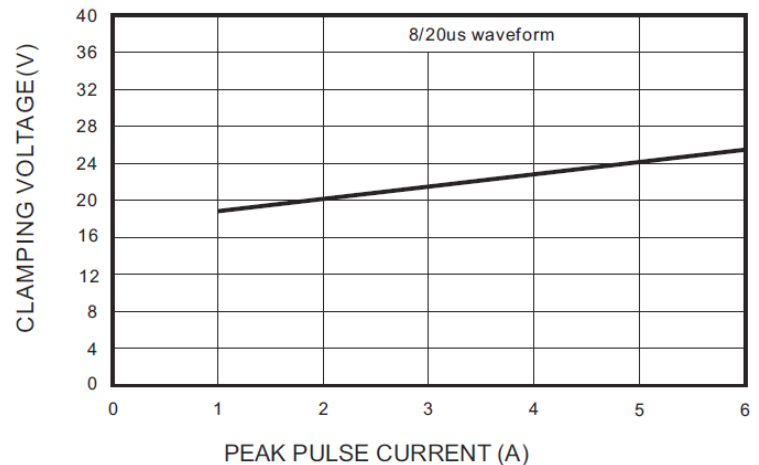
FIG.2- CLAMPING VOLTAGE VS. PEAK PULSE CURRENT
